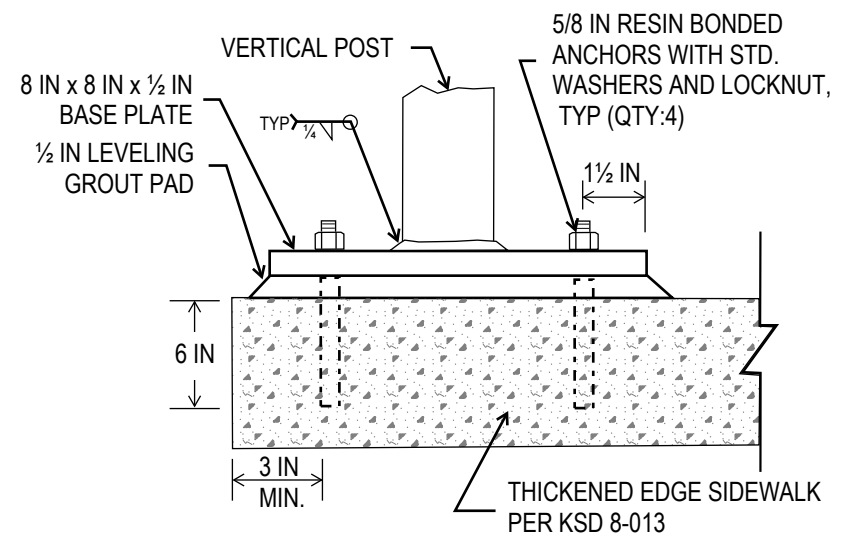
SURFACE MOUNT DETAIL
