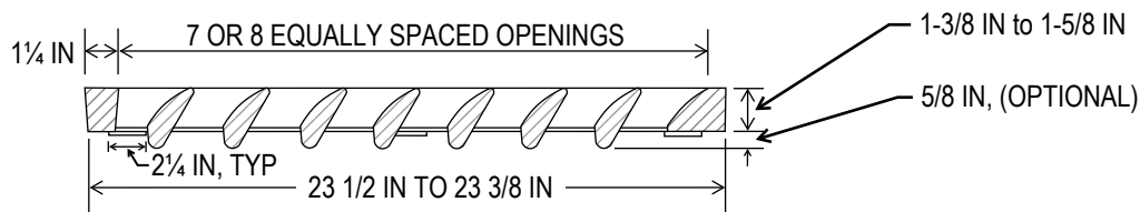
PROFILE VIEW
