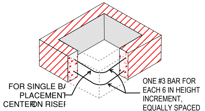
RISER REINFORCEMENT
