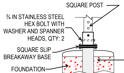
BREAKAWAY BASE DETAIL
