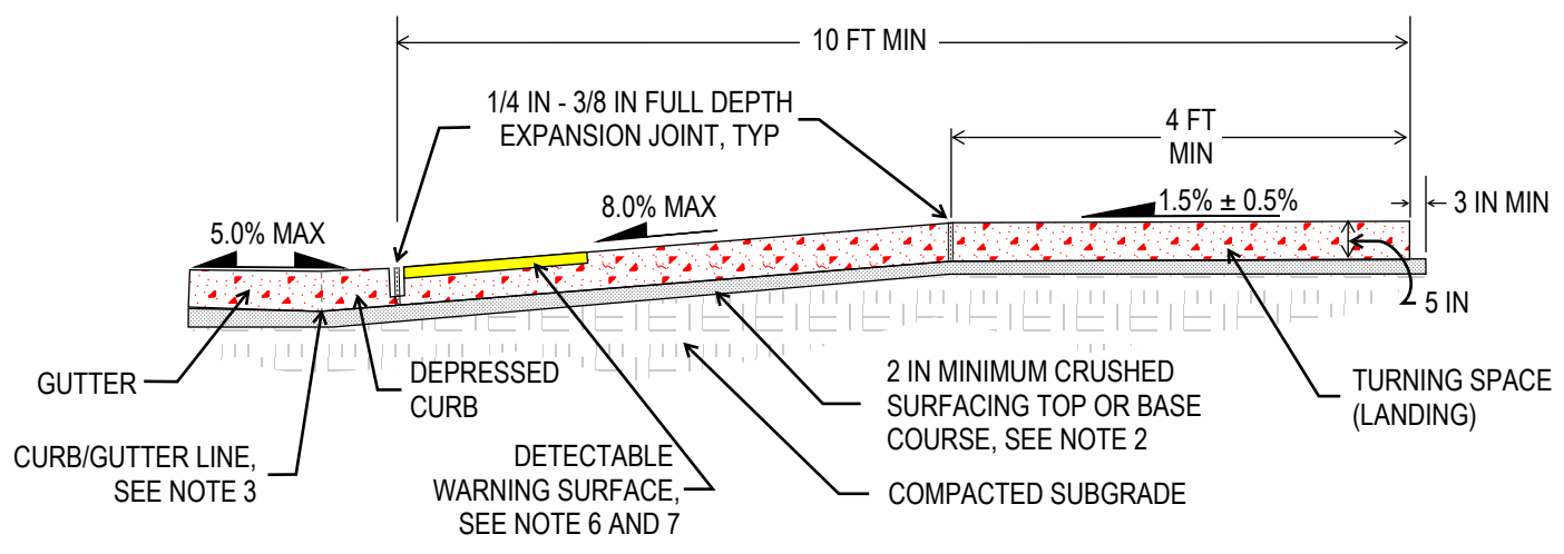
TURNING SPACE/RAMP CROSS SECTION
