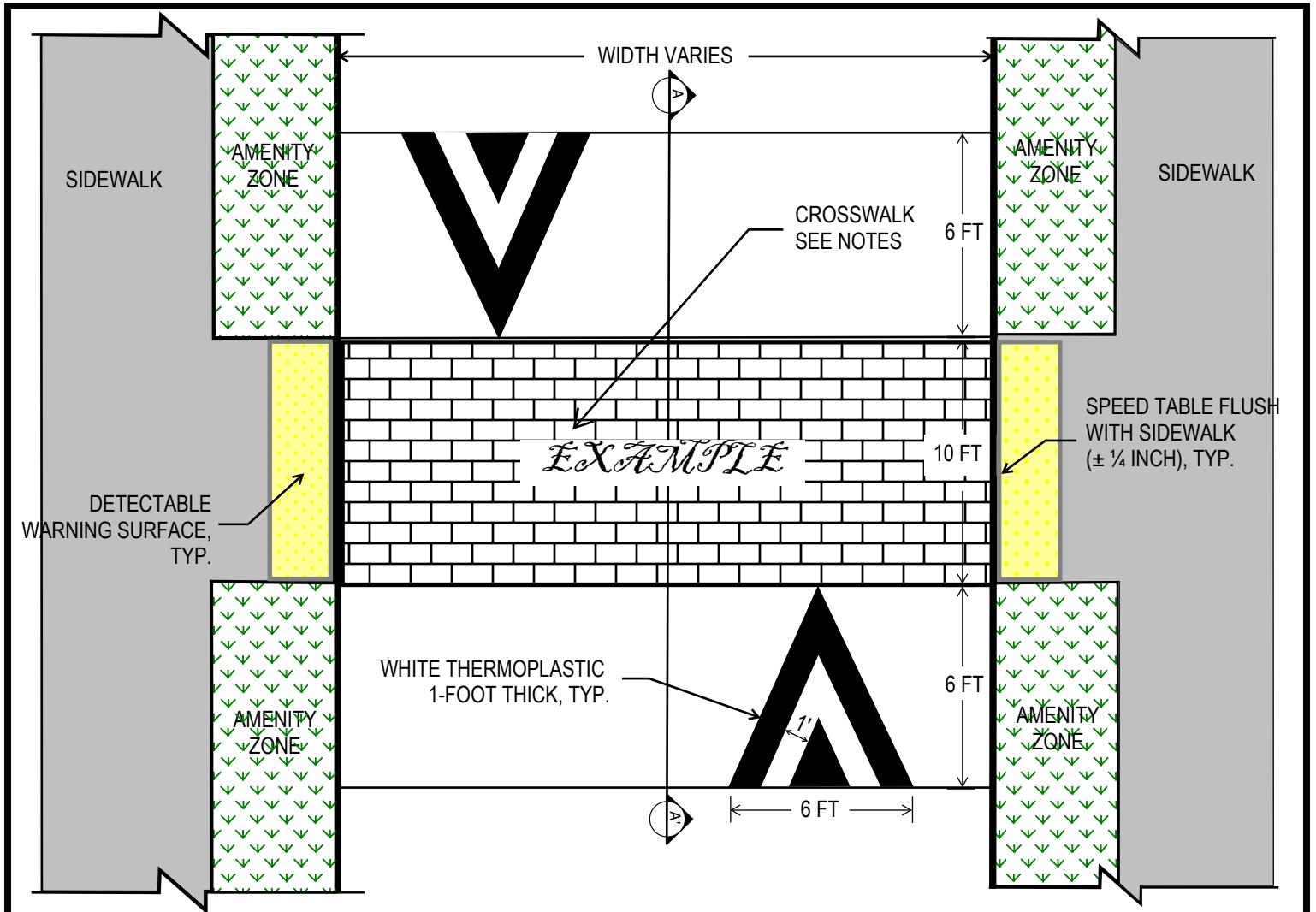
PLAN VIEW
