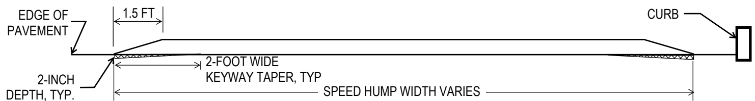
SECTION B-B'
