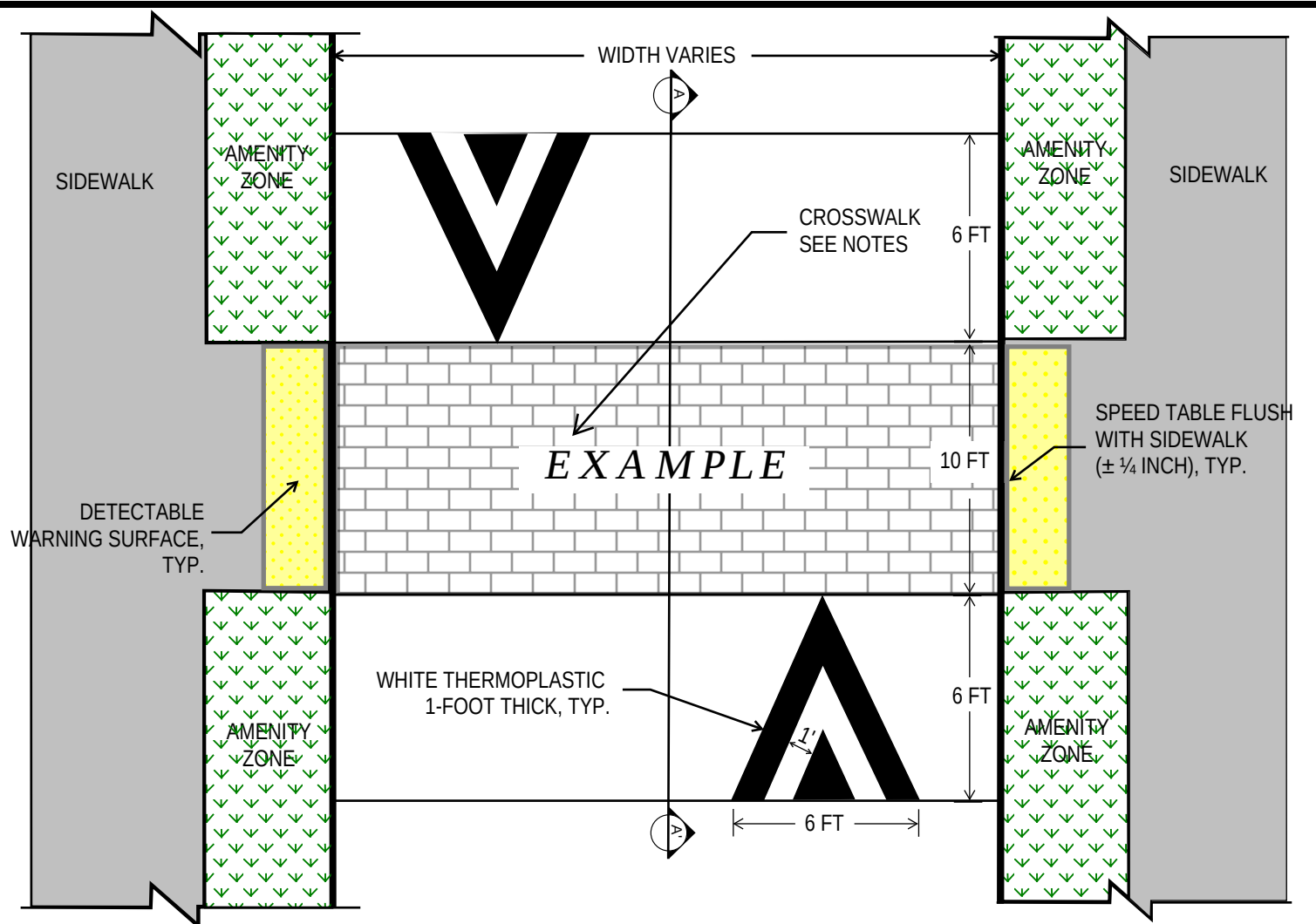
PLAN VIEW
