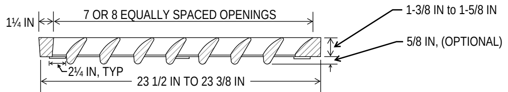
PROFILE VIEW
