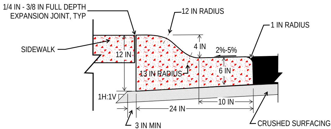
ROLLED CURB
