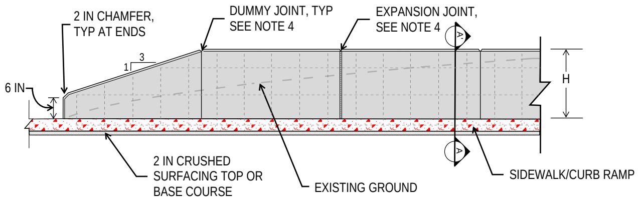
PROFILE VIEW
