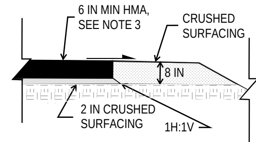
SHOULDER SECTION
