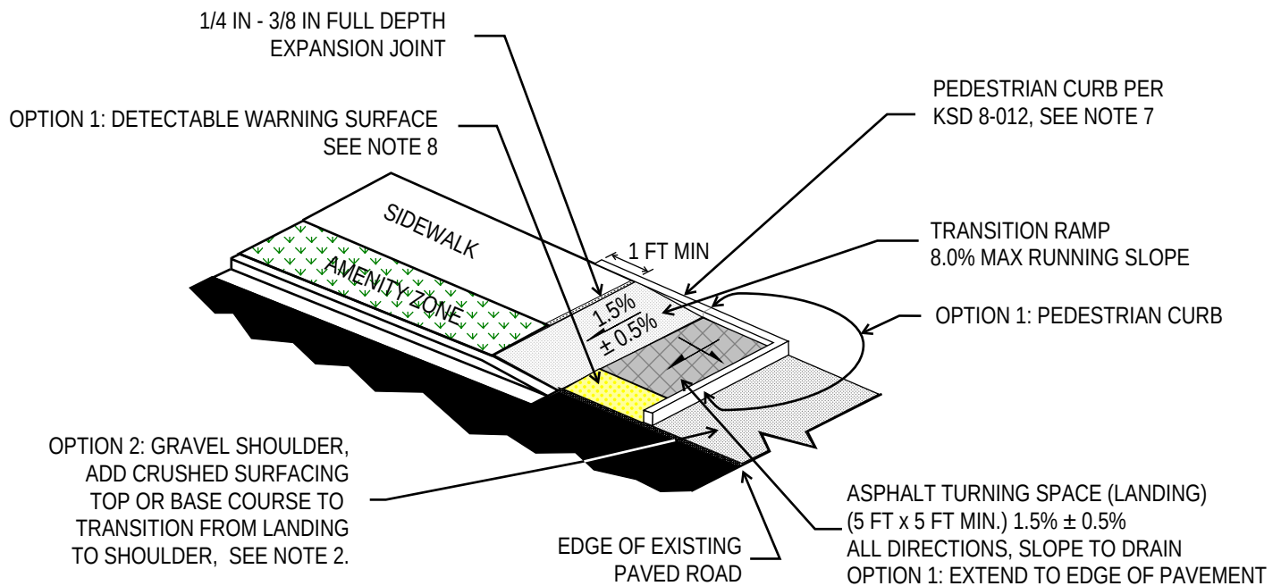
PLAN VIEW
