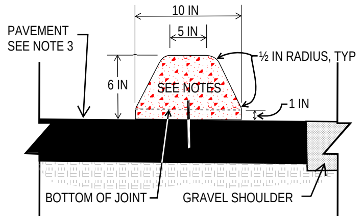
EXTRUDED CURB
