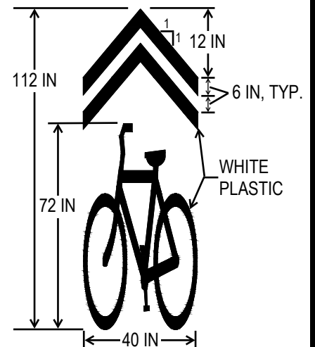
SHARROW SYMBOL
