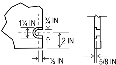
LOCKING BOLT DETAIL
