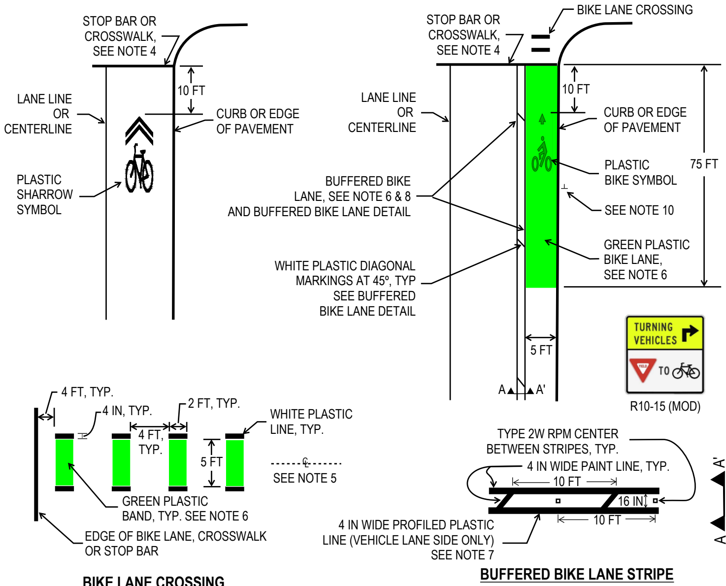
BIKE LANE CROSSING
