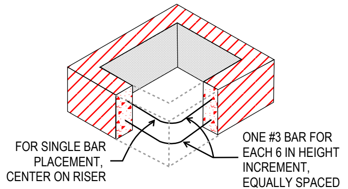
RISER REINFORCEMENT
